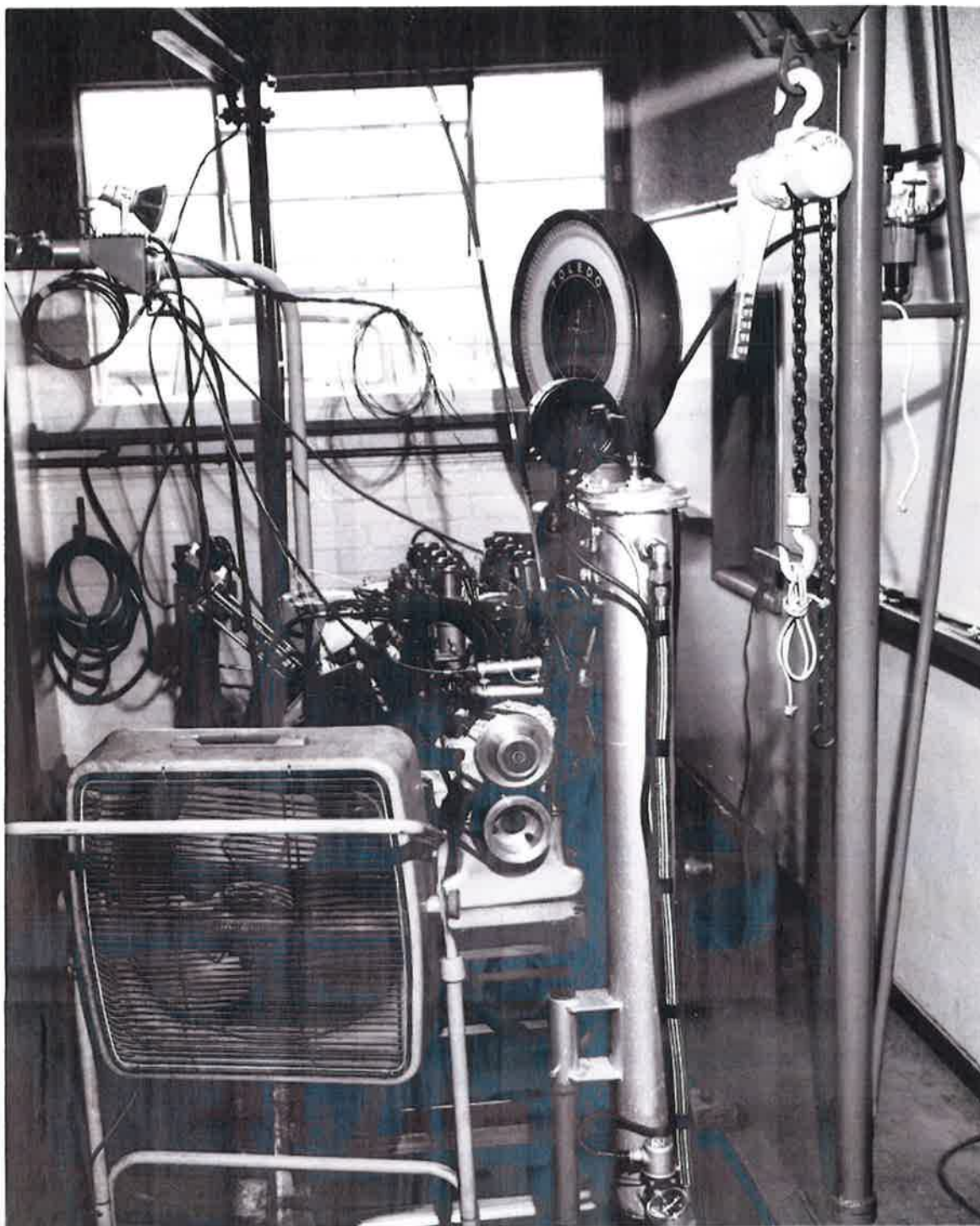
A Shelby American 260 cu in Ford (or early 289 HIPO) motor with 48 Weber IDA carburetors being run on a dynamometer in Venice, California in early 1963. Engines were modified and put to the test before being run in competition. (Robert Walker Collection)
